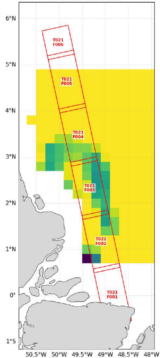
SMOS asc field (red = BIOMASS swath)
